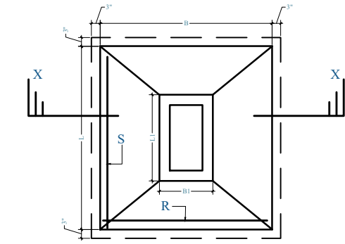
TYPICAL PLAN OF COLUMN FOOTING
