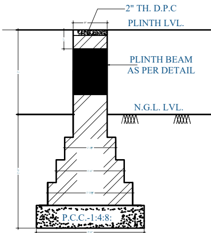
FOUNDATION OF 9" TH. BRICK WALL ( FW1 )
