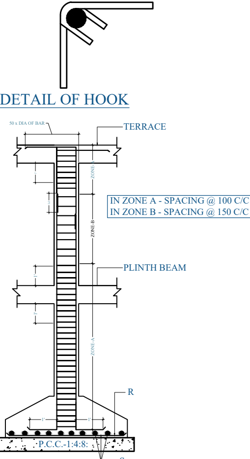
DUCTILITY DIAGRAM AS PER IS:13920
