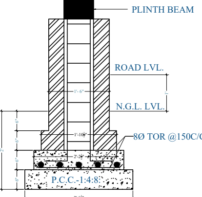
SECTION AT B-B
